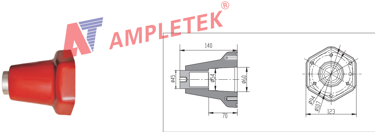
Type:ANC-1 (1# 内锥插座Inner cone socket)
